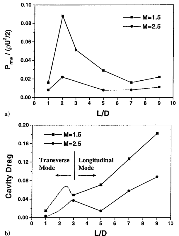
Fig. 6 Effect of L/D on a) magnitude (root mean square) of pressure fluctuations on the bottom of the cavity (at x/D = 0.33 ) and b) drag of the cavity at Mach 1.5 and 2.5 flows. 25
